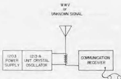
Figure 3. Arrangement of Unit Crystal Oscillator and receiver for standardization and use.
