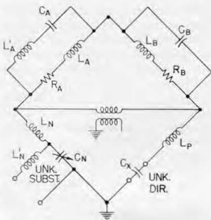
Figure 2. Simplified schematic diagram of Type 716-CS1, showing location of the more important residual inductances.
